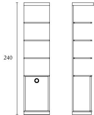
Cod. HMATBI104I2PB / Cod. HMATBI104I2PBL cm 104 x 46 x h 240 - inch 40.9 x 18.1 x 94.4
