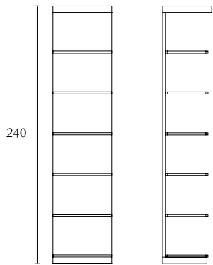
Cod. HMATBI104CV / HMATBI104CL / HMATBI104C cm 104 x 46 x h 240 - inch 40.9 x 18.1 x 94.4
