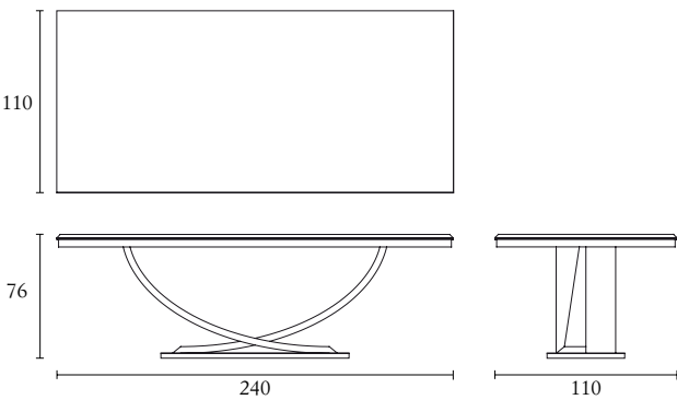
Cod. HATAB240B cm 240 x 110 x 76 - inch 94.4 x 43.3 x 30
