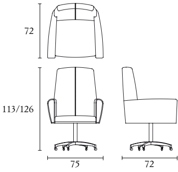
Cod. HAFAUBURG cm 75 x 72 x h 113/126 - inch 29.5 x 28.3 x 44.4/49.6
