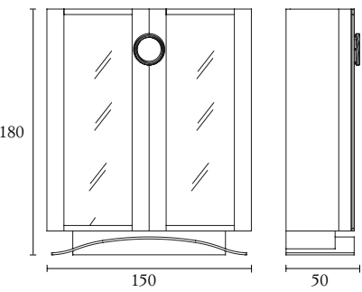
Cod. HACONS cm 180 x 38 x 74 - inch 70.8 x 15 x 29.1
