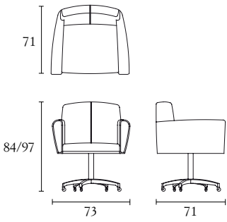
Cod. HAFAUBURP cm 73 x 71 x h 84/97 - inch 28.7 x 27.9 x 33/38.2
