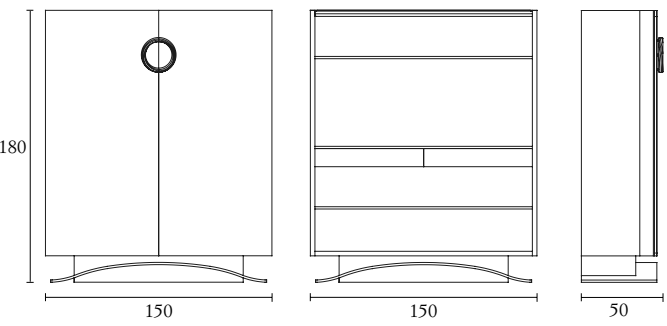
Cod. HAUSSBAR cm 150 x 50 x 180 - inch 59 x 19.6 x 70.8
