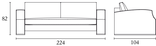
Cod. ANTOI280SM cm 284 x 104 x h 82 - inch 110 x 40.9 x 32.2
