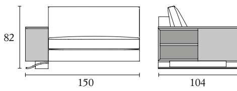
Cod. HAUSSMON210SM cm 210 x 104 x h 82 - inch 82.6 x 41 x 32.2
